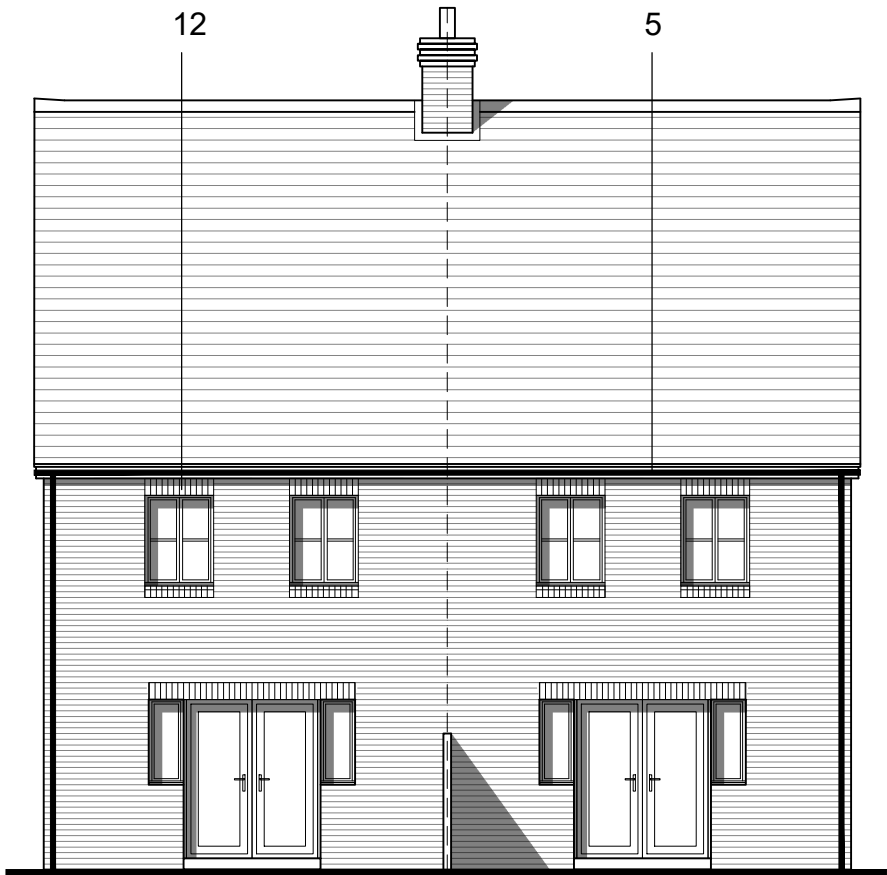
Proposed Rear (West) Elevation
