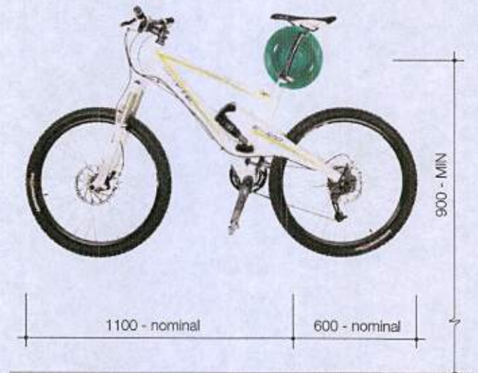
Single bike horizontal - seat post
