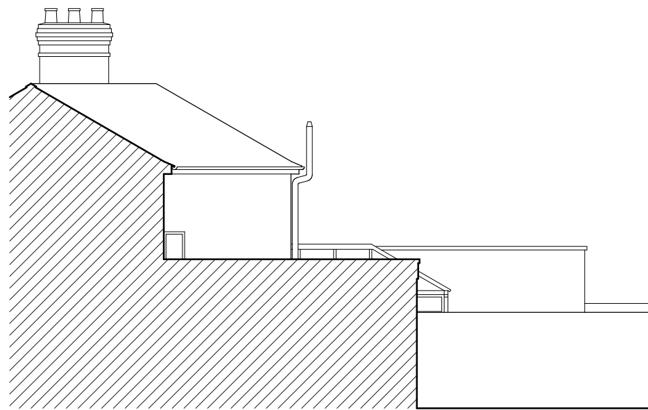
West Elevation C C
