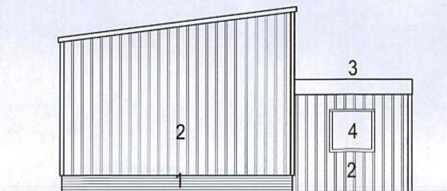
NORTH ELEVATION
