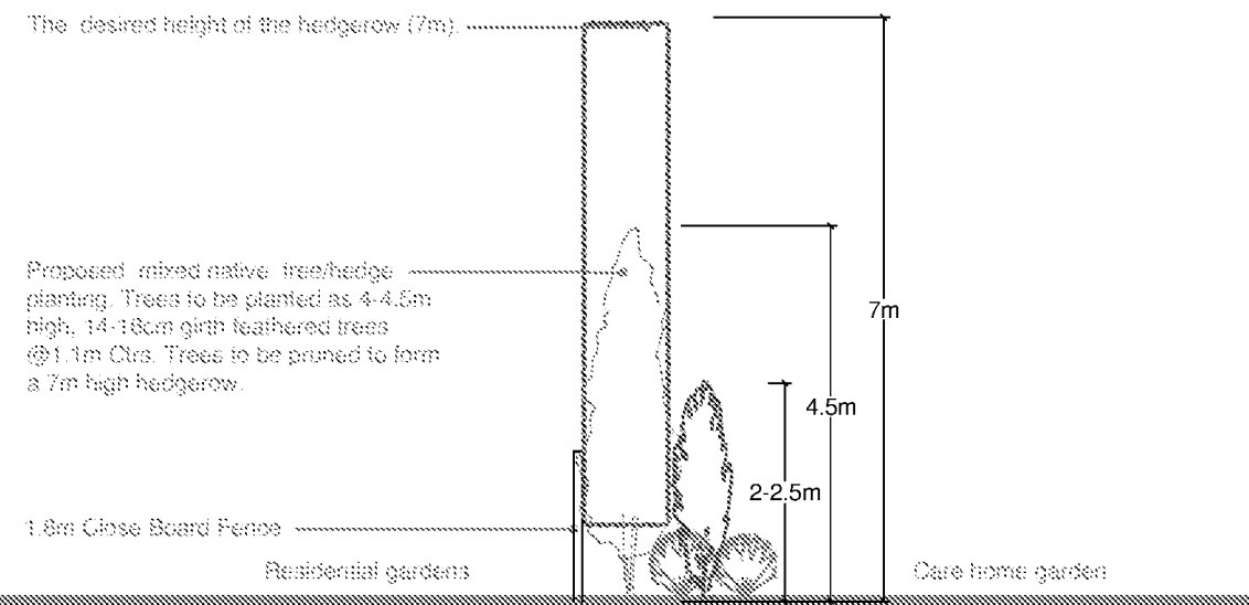
Section View B-B SCALE: 1:100@A1
