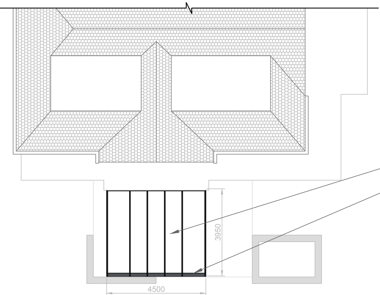
Roof Plan
