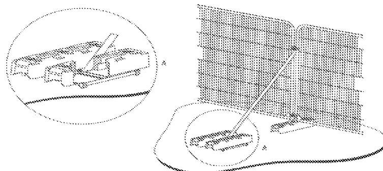
b) Stabilizer strut mounted on block tray
