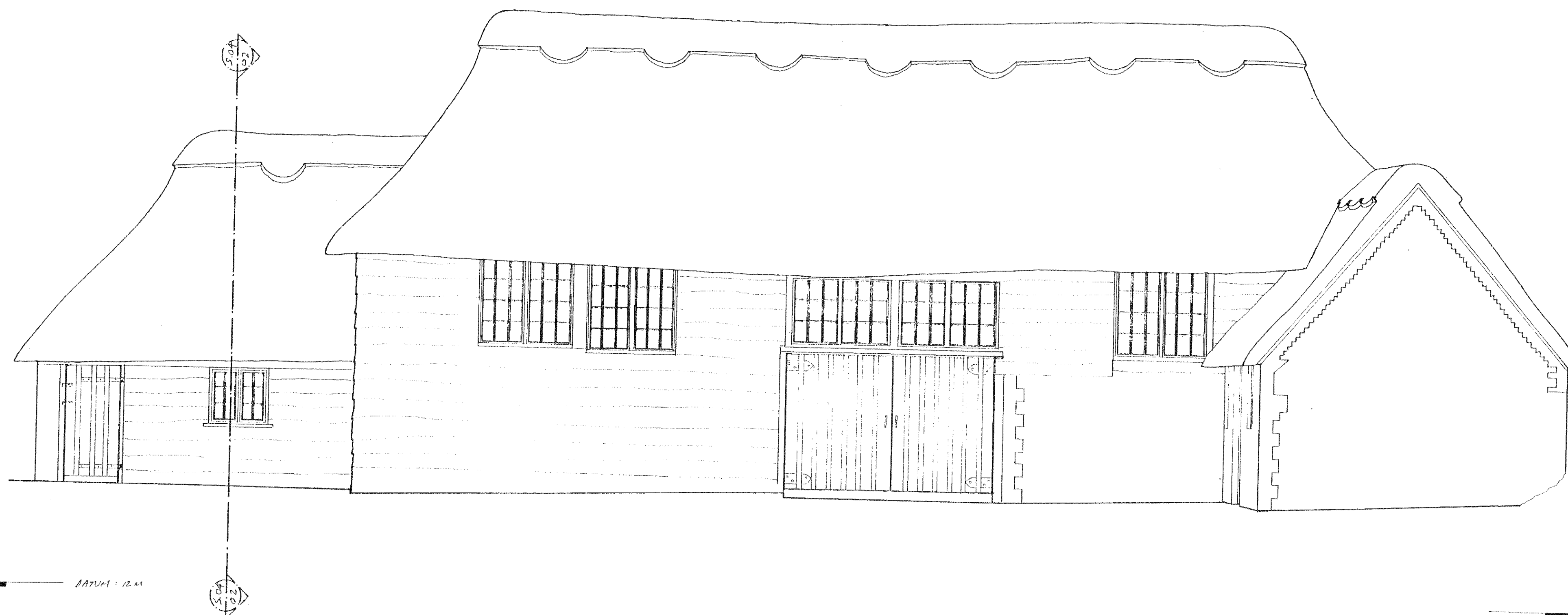
01 BARN : SOUTH ELEVATION 1:50
