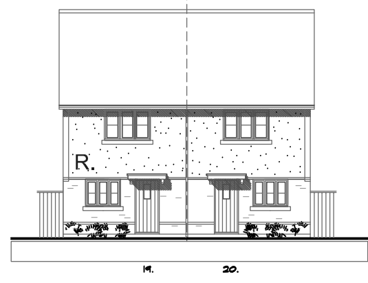
FRONT ELEVATION - West [3 BEDROOM] Semi-detached houses PLOTS 19 & 20
