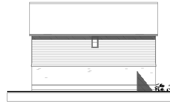
SIDE ELEVATION - East
