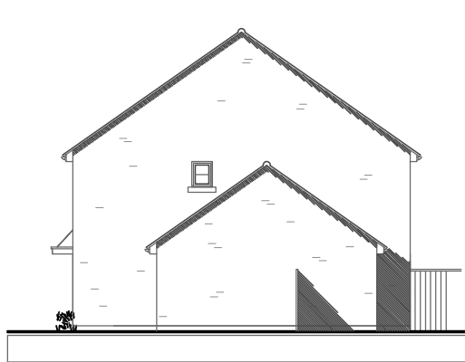
1. SIDE ELEVATION - East Inner East & West Elevations Plots 2/3 similar
