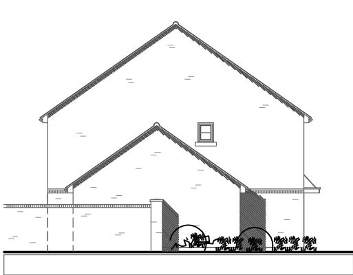
4. SIDE ELEVATION - West [2 BEDROOM] Semi-detached houses with garage
