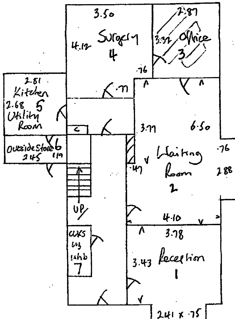
GROUND FLOOR
