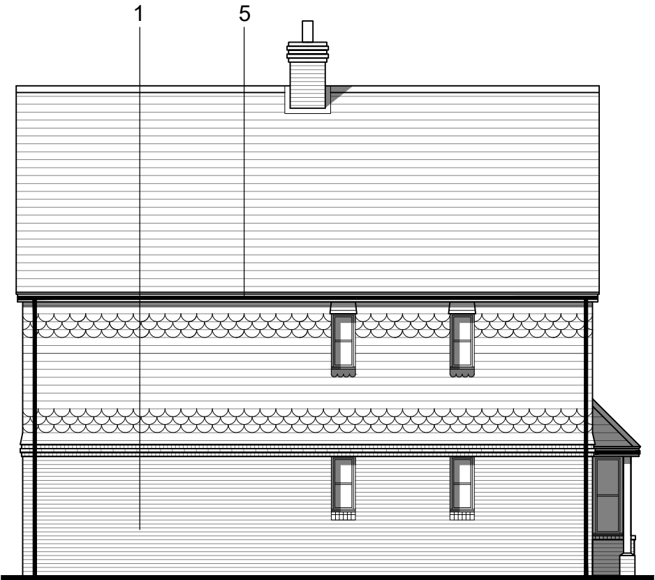
Proposed Side (South) Elevation
