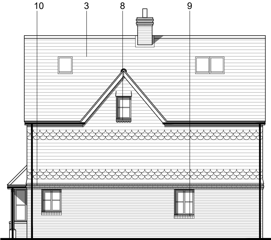
Proposed Side (North) Elevation
