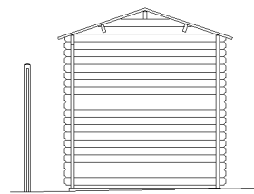
Side (North)
