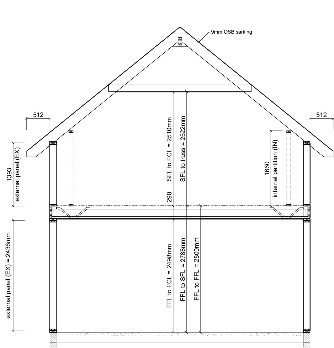
Section E-E
