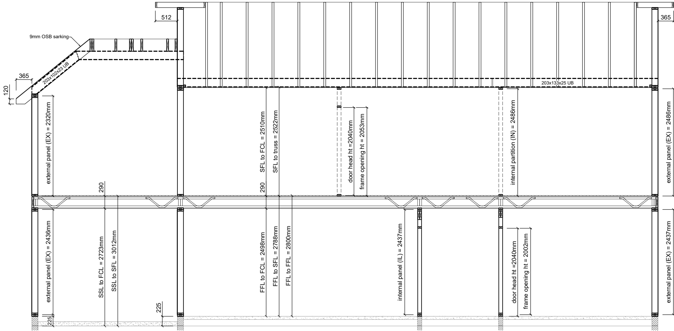
Section F-F
