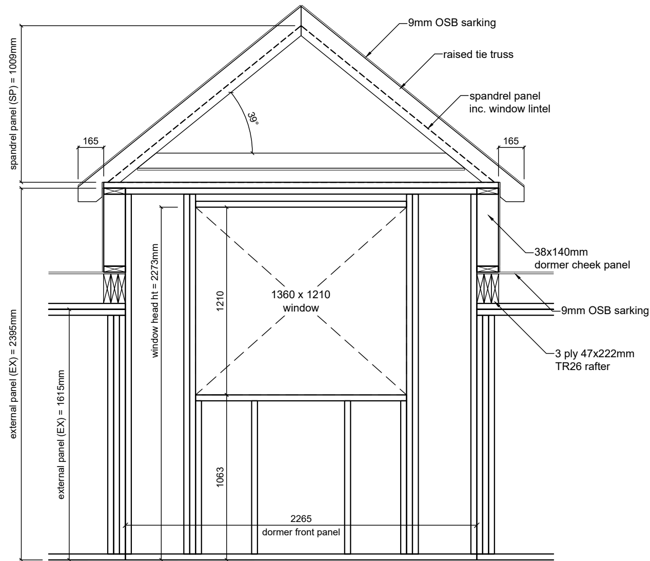
Dormer Elevation (Bed 2) (1:25)
