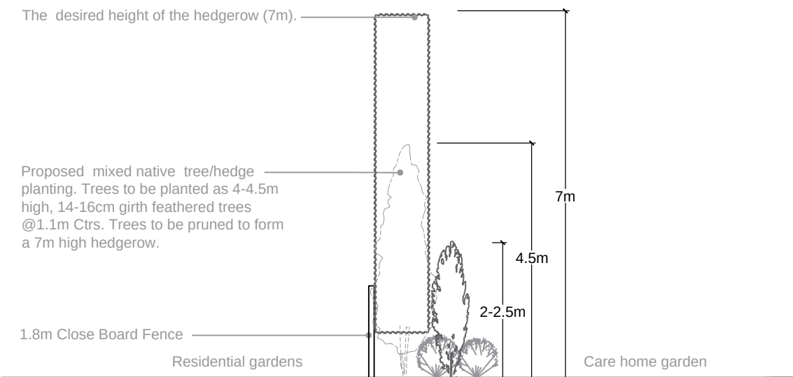
Section View B-B SCALE: 1:100@A1
