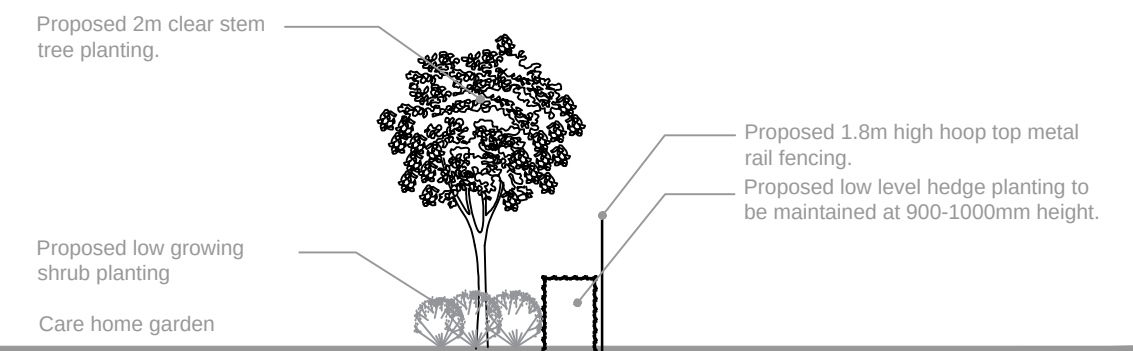
Section View C-C SCALE: 1:100@A1
