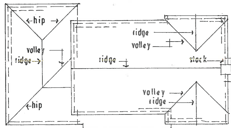
ROOF PLAN 1/200
