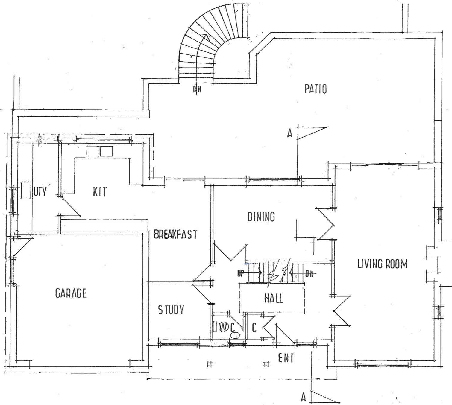
GROUND FLOOR 1/100
