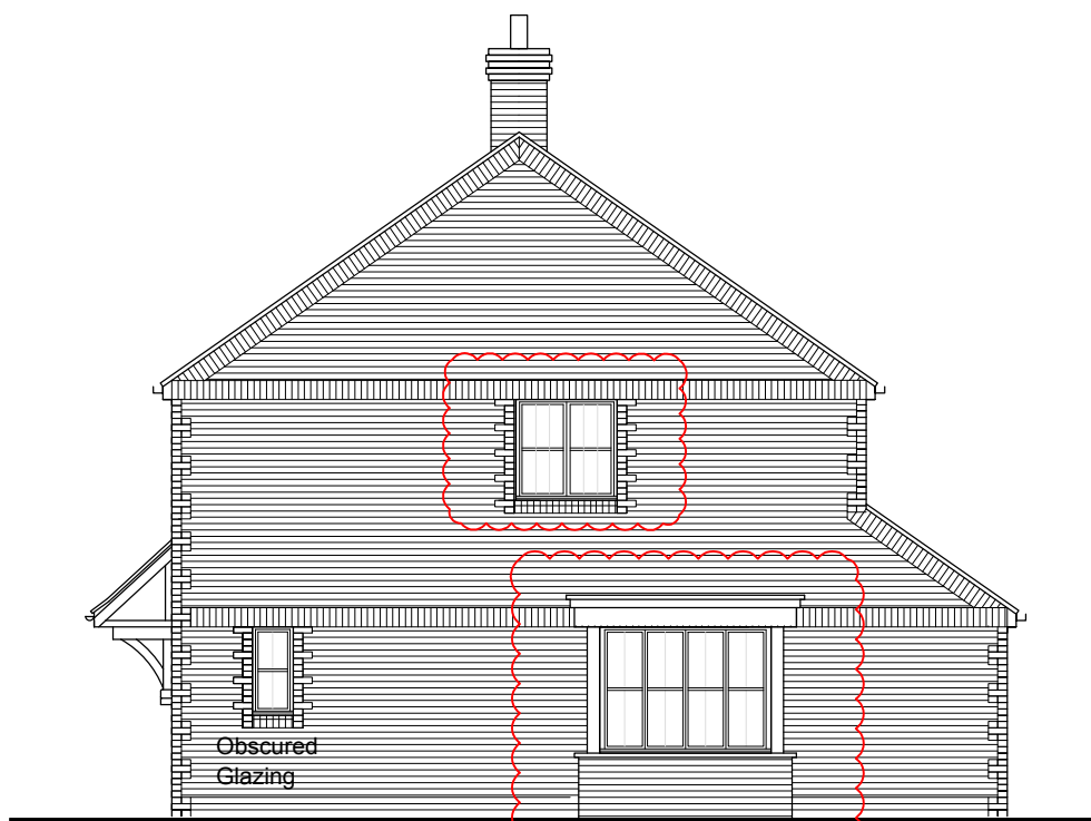
Side Elevation 2
