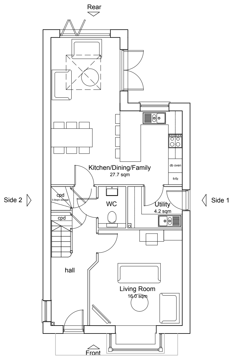
Ground Floor Plan 3-Bedroom 5-Person House 115.5 sqm / 1243 sqft GIA (to finishes) 2.5sqm storage required
