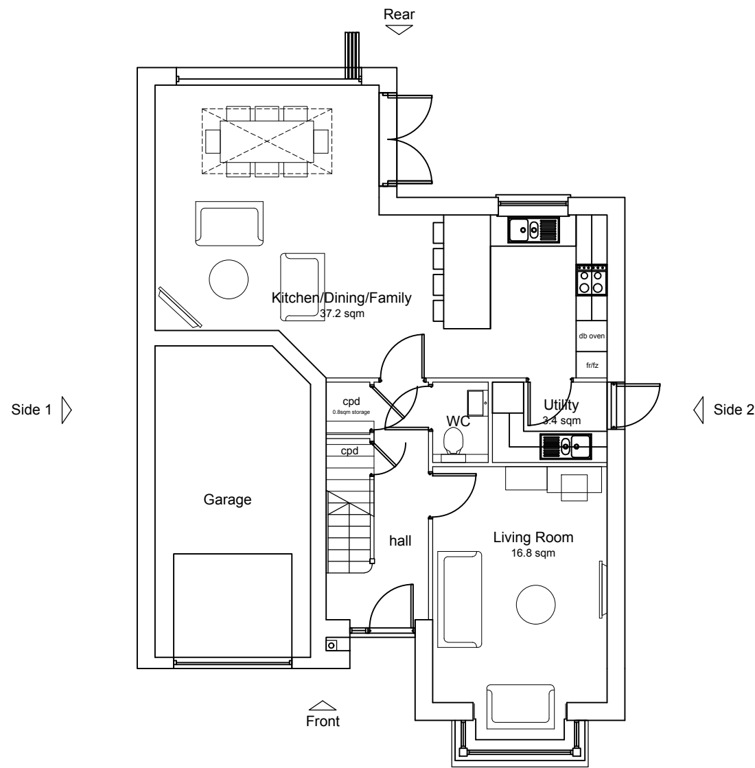
Ground Floor Plan 4-Bedroom 8-Person House 144 sqm / 1550 sqft GIA (to finishes)
