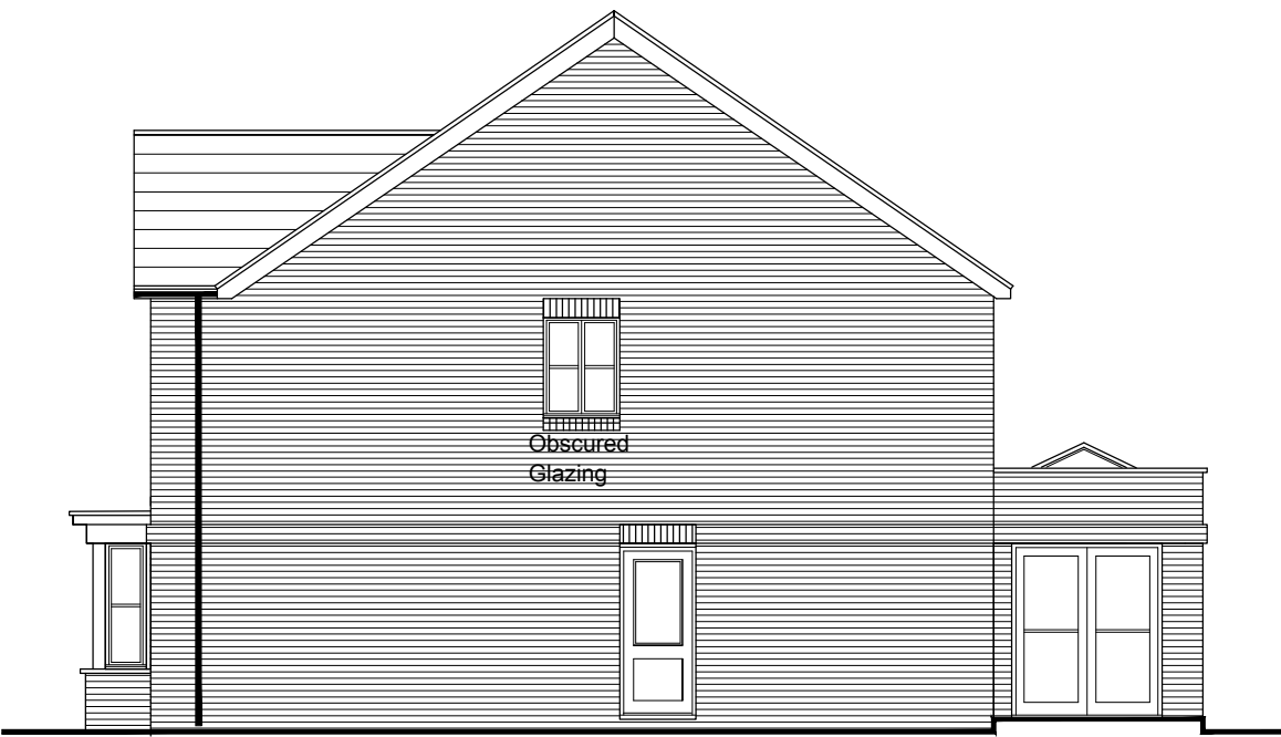
Side Elevation 2
