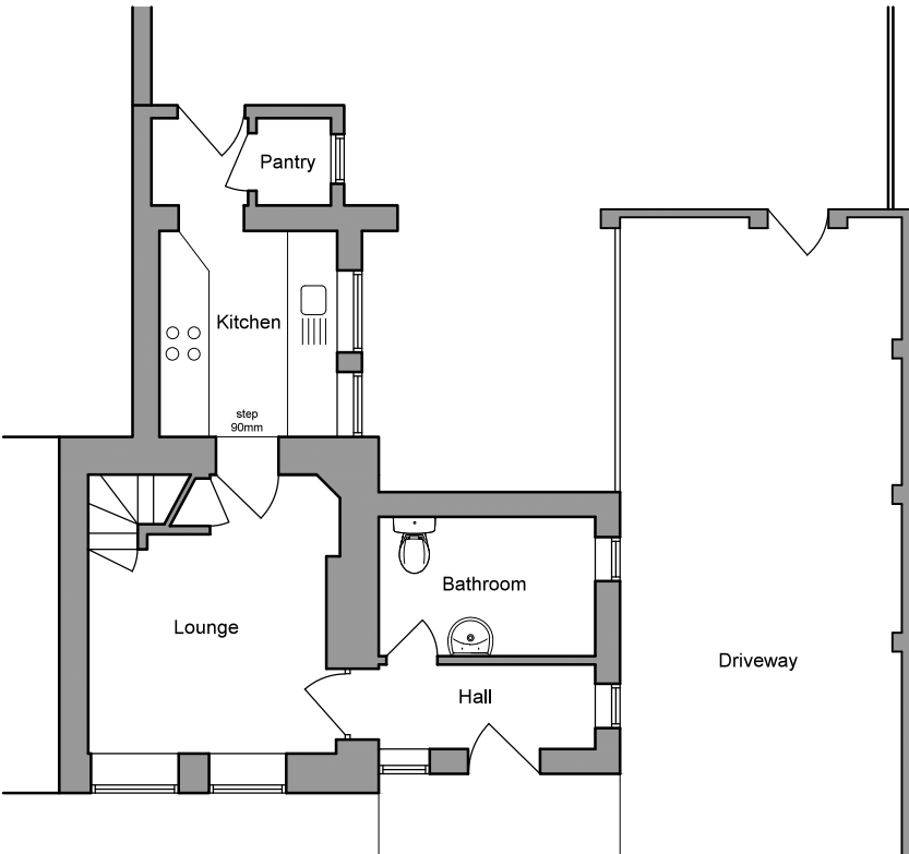
GF PLAN 1:100@A3
