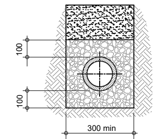
GRANULAR SURROUND (CLASS S) To be used where cover to crown of pipe is greater than 600mm under private soft landscaped areas and greater than 900mm under drives. Concrete bed and surround to be used elsewhere
