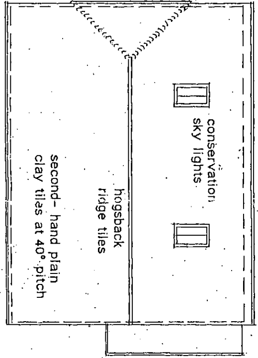
ROOF PLAN
