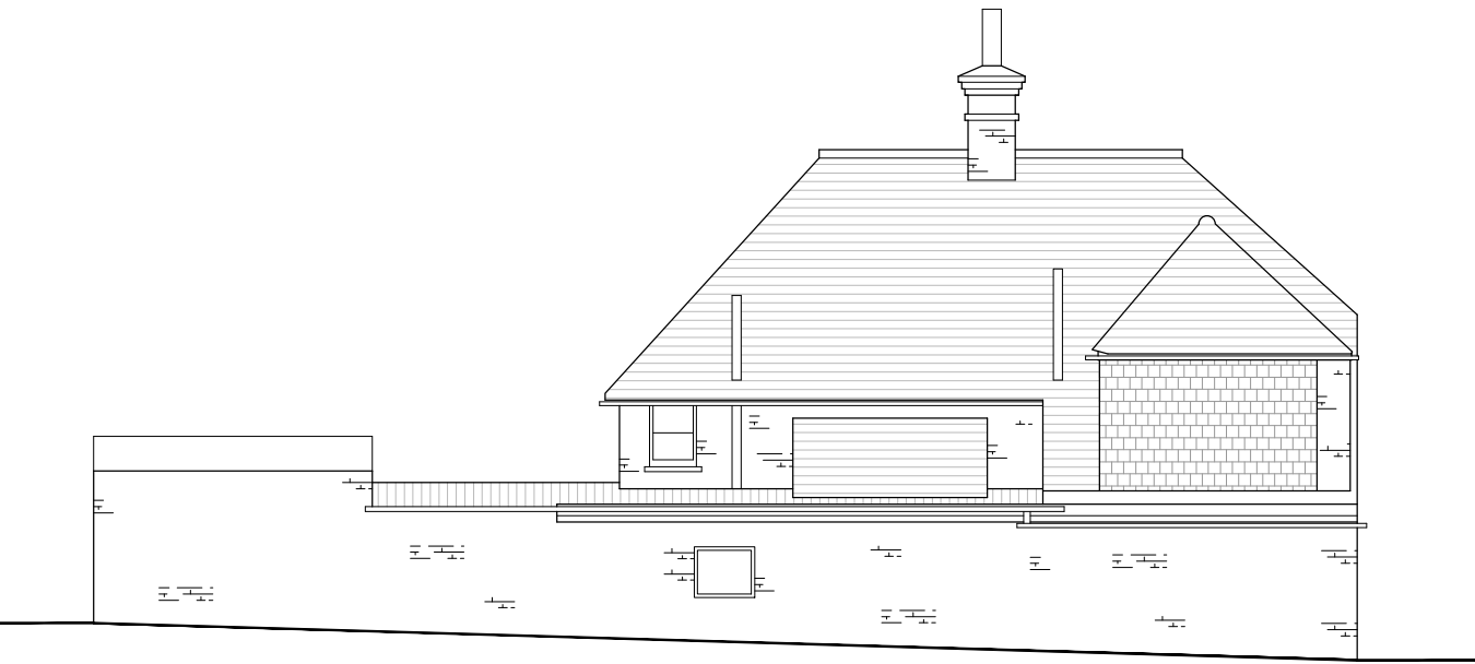
EXISTING SOUTH ELEVATION SCALE 1:100
