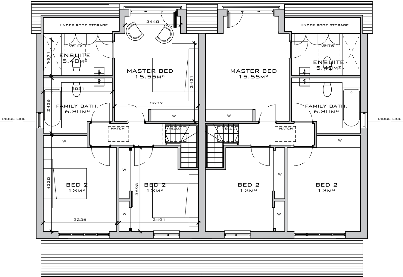
FIRST FLOOR PLAN - OPT 1 1:100 SCALE @ A3
