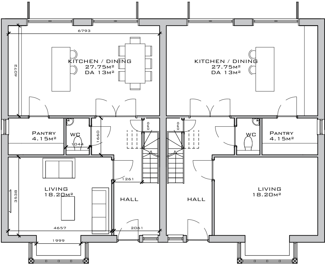
GROUND FLOOR PLAN - OPT 1 1:100 SCALE @ A3
