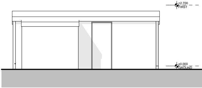
GARAGE WEST ELEVATION 1:100
