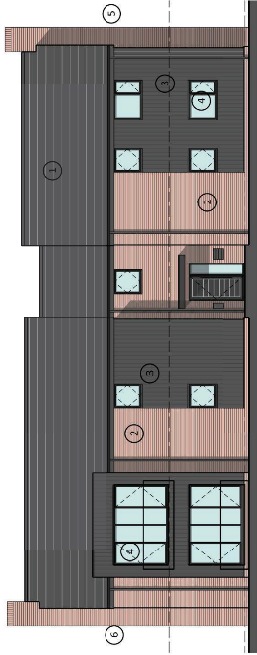
Front Elevation GF: Plot 3 FF: Plot 5
