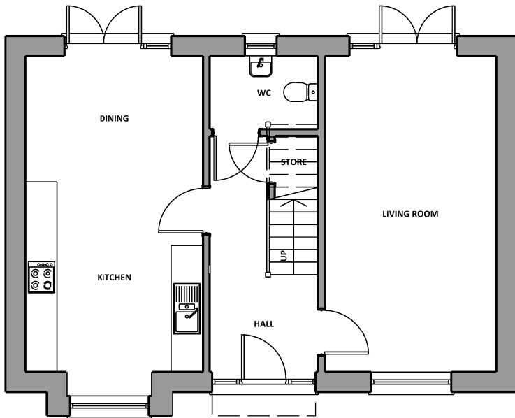
Ground Floor Plot 31 & 68 3 Bed 6 Person GF GIA: 51.80sqm Total GIA: 105.20sqm Private
