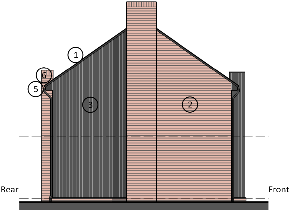
Gable Elevation GF Plot 48 FF Plot 50
