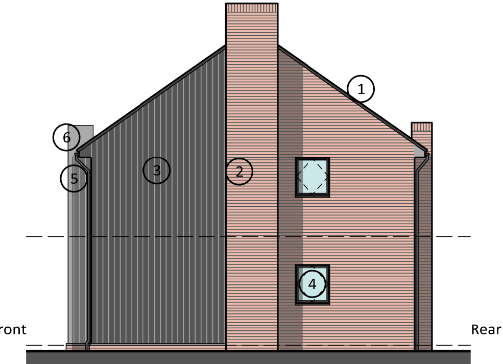
Gable Elevation GF Plot 49 FF Plot 51
