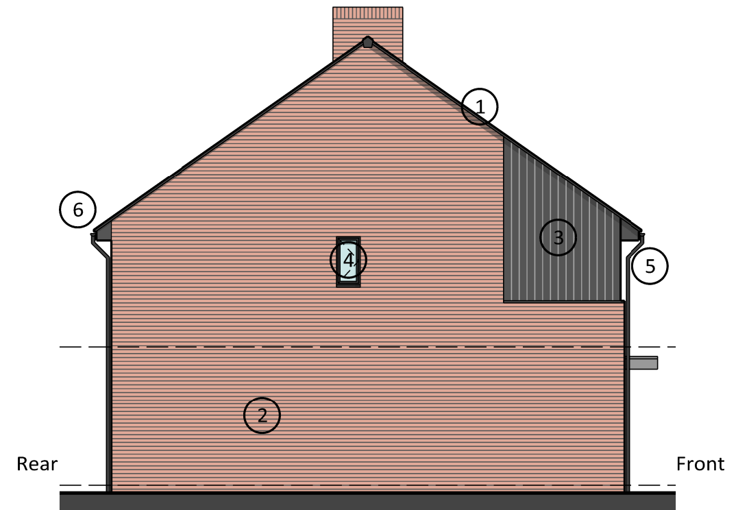
Gable Elevation Plot 30
