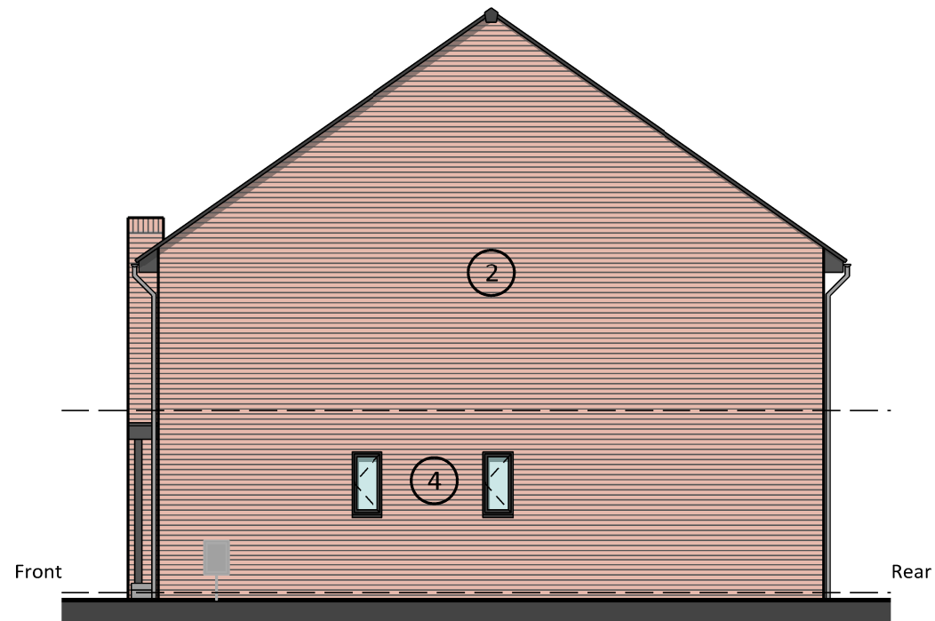
Gable Elevation Plots 63, 65 & 67 Plots 70, 72, 74 & 76
