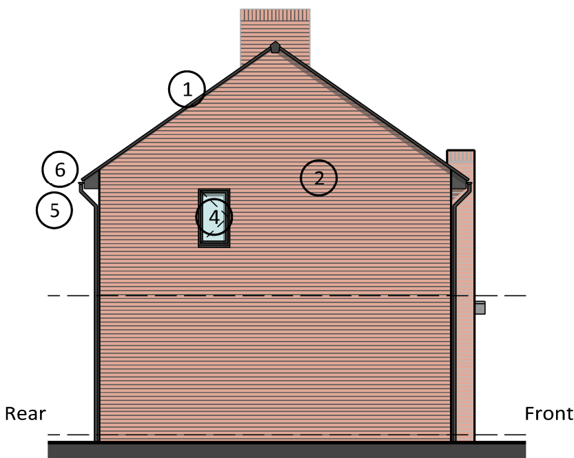
Gable Elevation Plot 25
