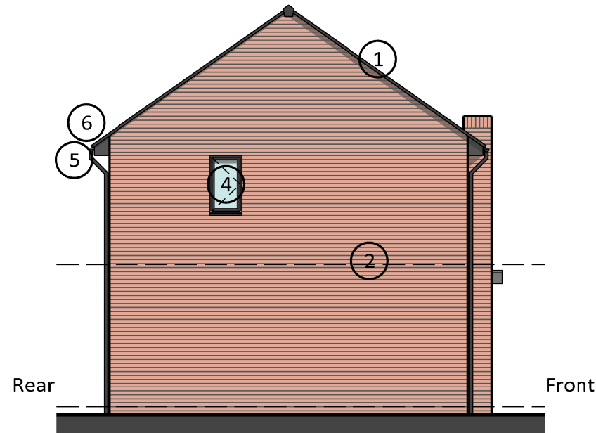
Gable Elevation Plot 31 & 68
