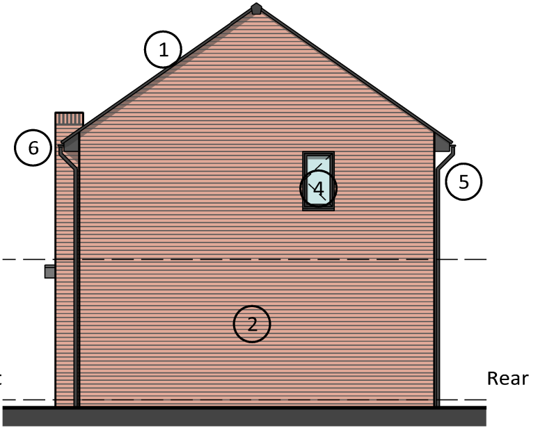
Gable Elevation Plot 21
