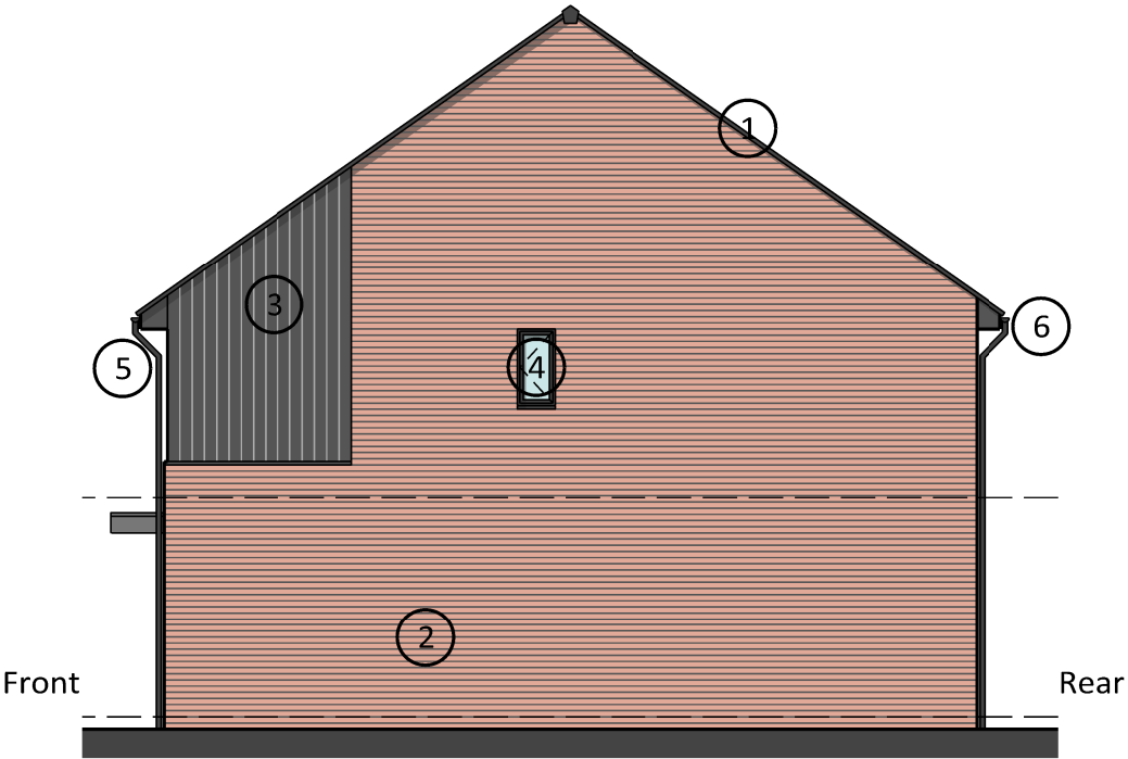
Gable Elevation Plot 15
