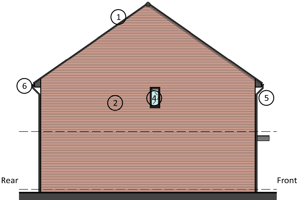
Gable Elevation Plot 13
