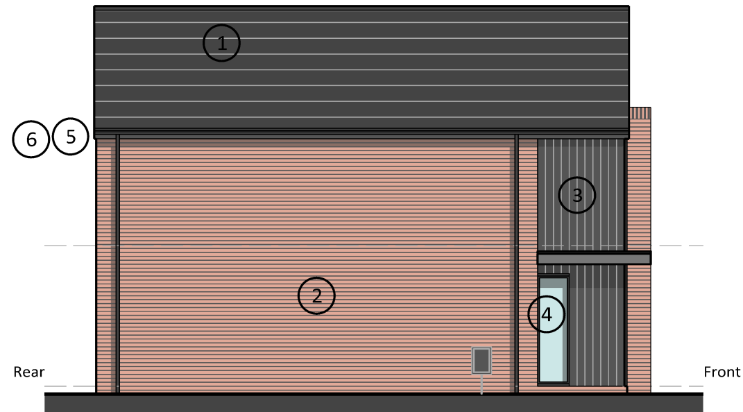
Gable Elevation Plots 22, 23 & 24
