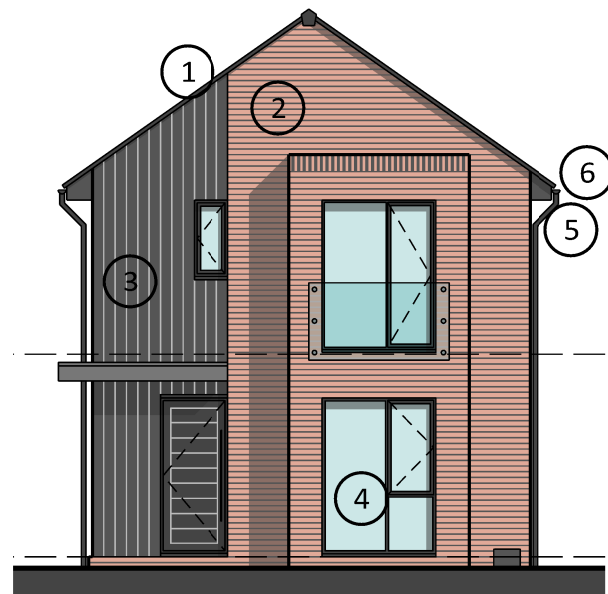
Front Elevation Plots 22, 23 & 24
