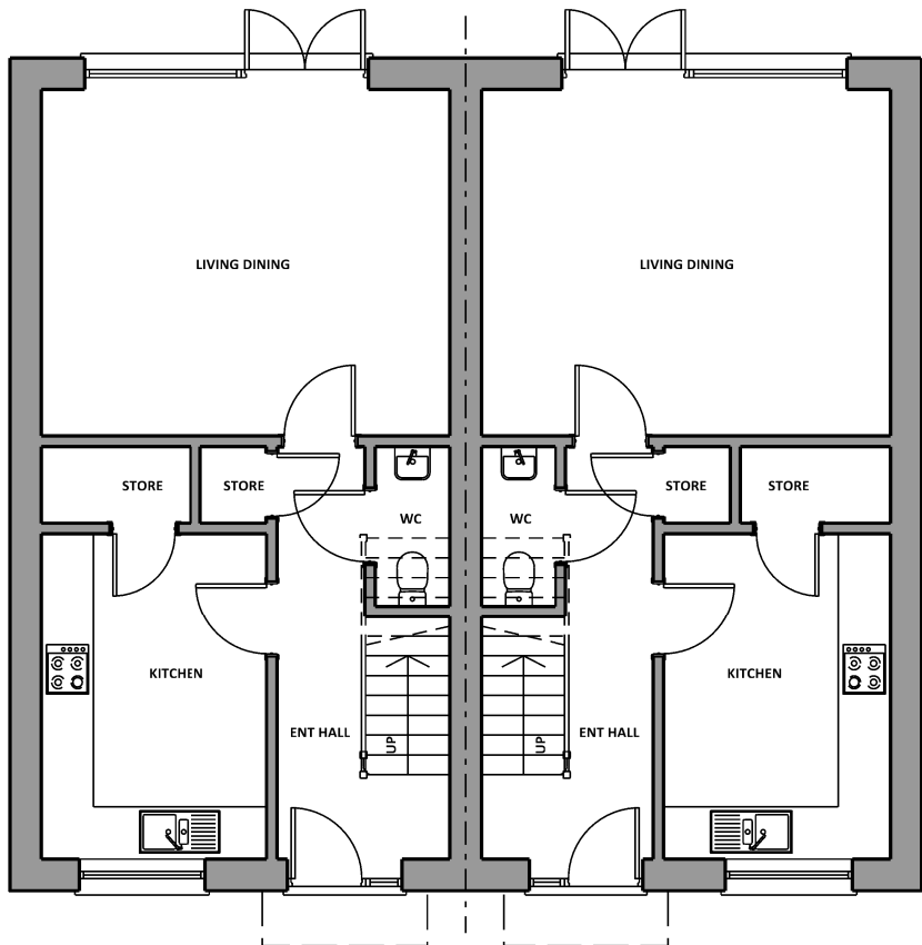
Ground Floor Plots 40, 42, 60, 77 & 87 2 Bed 4 Person GF GIA: 42.49sqm Total GIA: 87.00sqm Private
