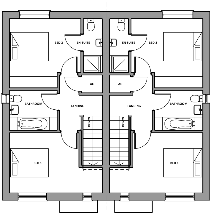
First Floor Plots 40, 42, 60, 77 & 87 FF GIA: 44.51sqm
