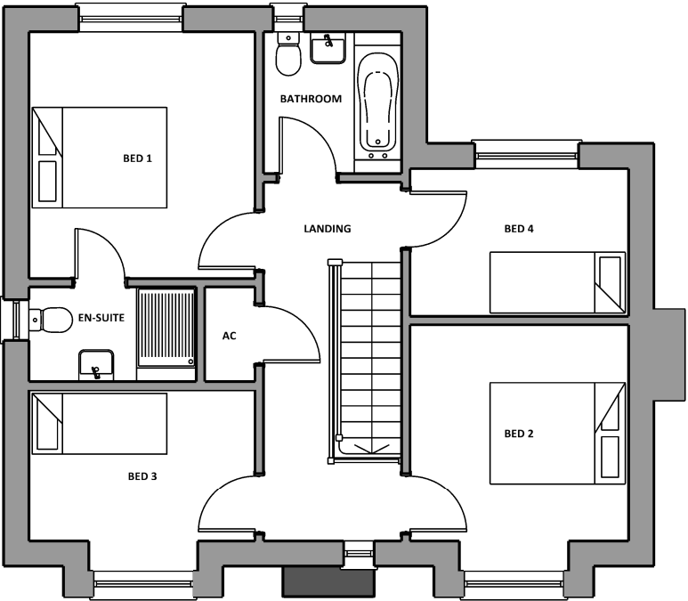
First Floor Plot 90 FF GIA: 62.07sqm
