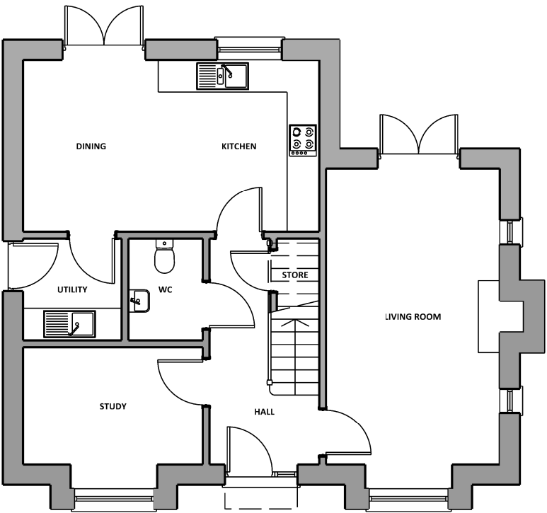
Ground Floor Plot 90 4 Bed 6 Person GF GIA: 60.47sqm Total GIA: 122.54sqm Private
