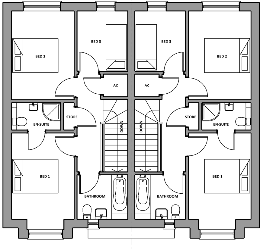
First Floor Plots 62, 64 & 66 Plots 69, 71, 73 & 75 FF GIA: 47.31sqm
