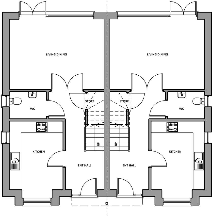
Ground Floor Plots 62, 64 & 66 Plots 69, 71, 73 & 75 3 Bed 5 Person GF GIA: 45.31sqm Total GIA: 92.62sqm Private
