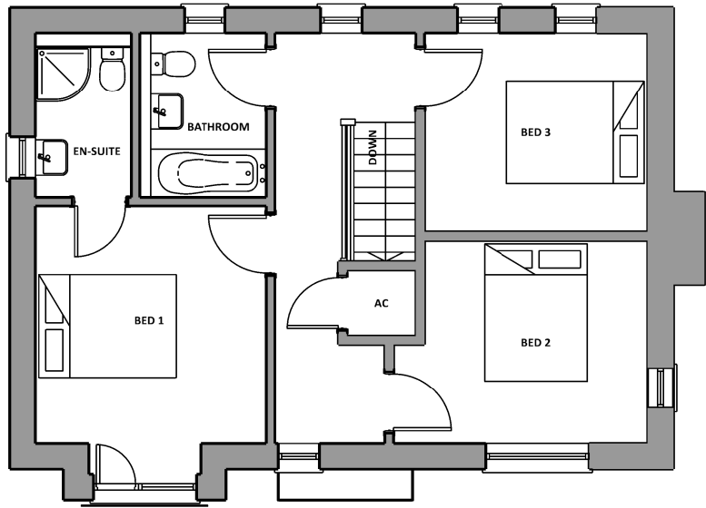
First Floor Plot 89 FF GIA: 54.13sqm
