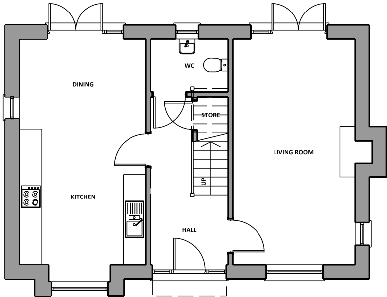
Ground Floor Plot 89 3 Bed 6 Person GF GIA: 52.53sqm Total GIA: 106.66sqm Private
