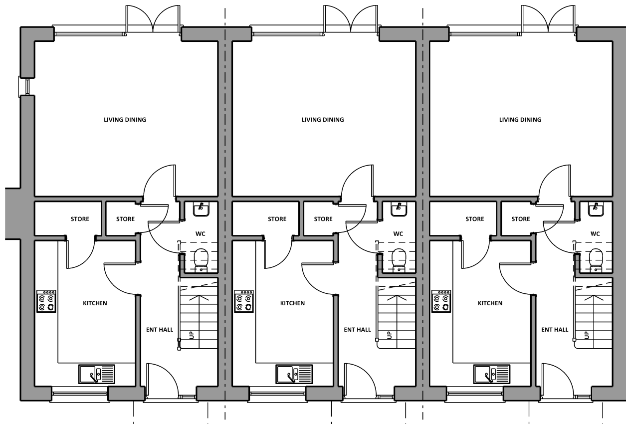
Ground Floor Plot 37 2 Bed 4 Person GF GIA: 42.49sqm Total GIA: 87.00sqm Private
