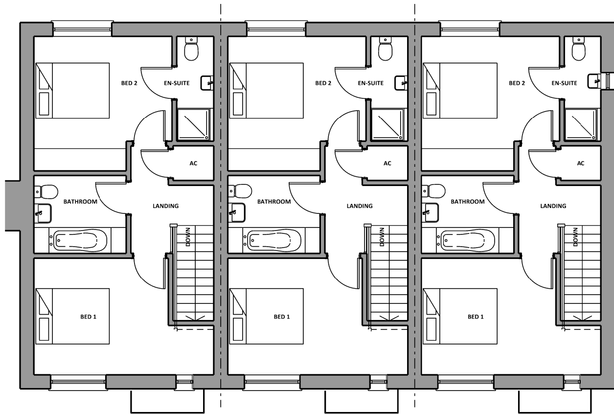
First Floor Plot 37 FF GIA: 44.51sqm
