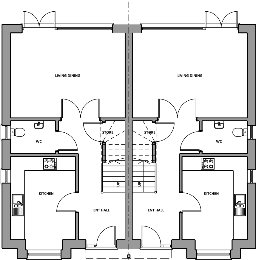
Ground Floor Plot 38 3 Bed 5 Person GF GIA: 45.31sqm Total GIA: 92.62sqm Private Ground Floor Plot 39 3 Bed 5 Person GF GIA: 45.31sqm Total GIA: 92.62sqm Private
