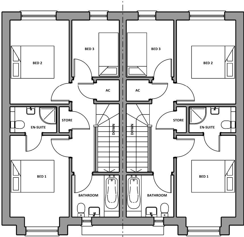
First Floor Plot 38 FF GIA: 47.31sqm First Floor Plot 39 FF GIA: 47.31sqm
