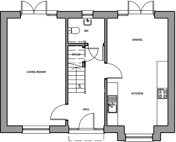
Ground Floor Plot 21 3 Bed 6 Person GF GIA: 51.80sqm Total GIA: 105.20sqm Private
