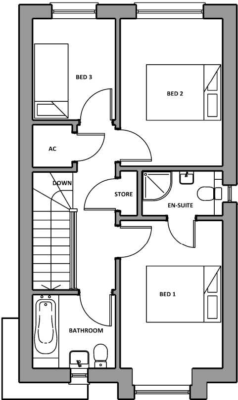
First Floor Plots 22, 23 & 24 FF GIA: 48.45sqm
