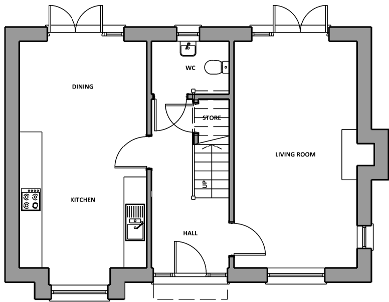
Ground Floor Plot 25 3 Bed 6 Person GF GIA: 51.80sqm Total GIA: 105.20sqm Private
