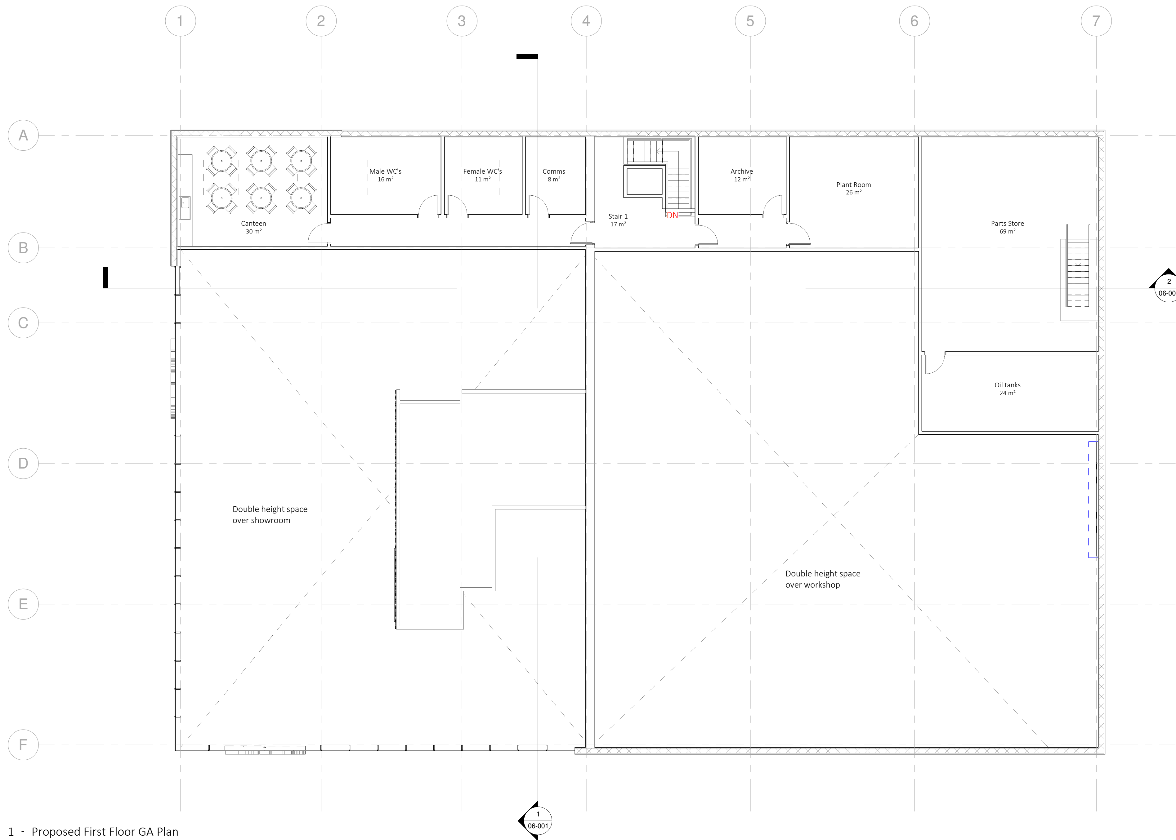
1 - Proposed First Floor GA Plan 1 : 100
