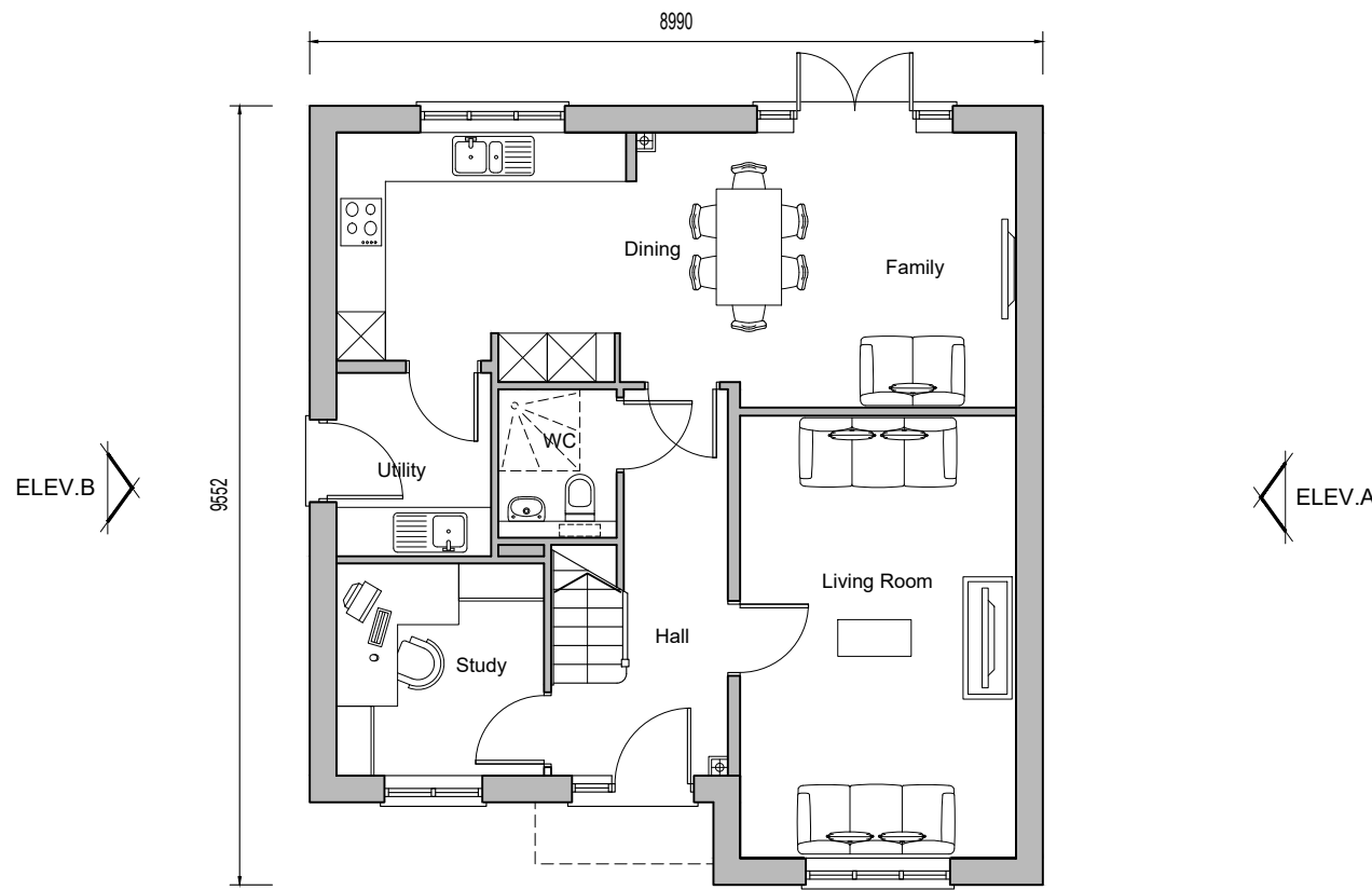
Ground Floor Plan Plot 507
