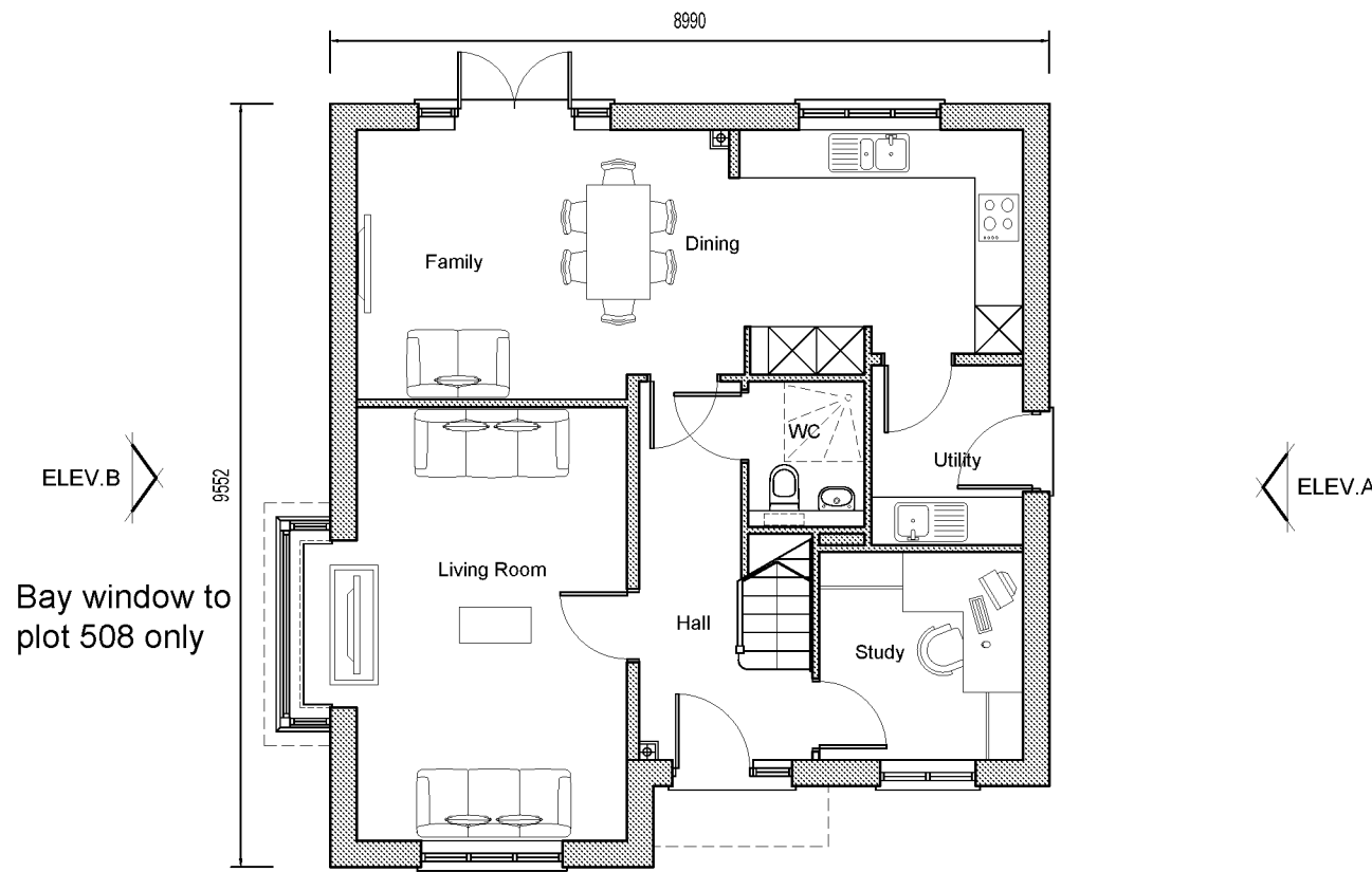
Ground Floor Plan Plot 508 Plot 501 (handed)
