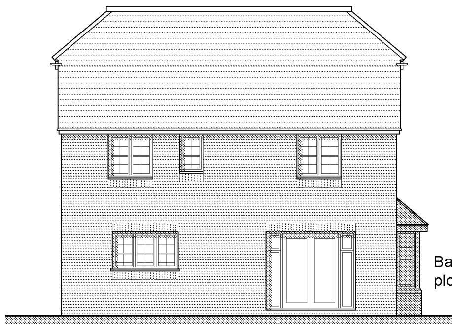
Rear Elevation
