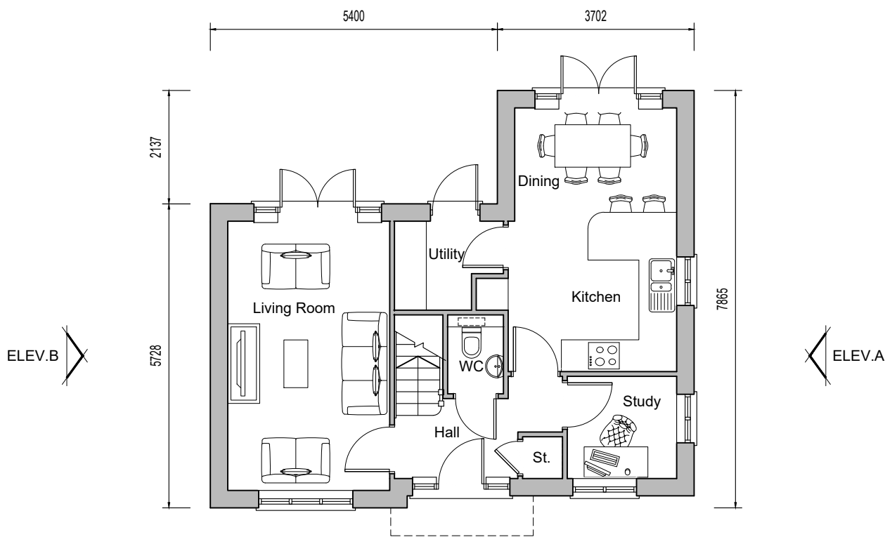
Ground Floor Plan Plots 356, 370, 394, 511 & 517 Plots 375 & 416 (handed)
