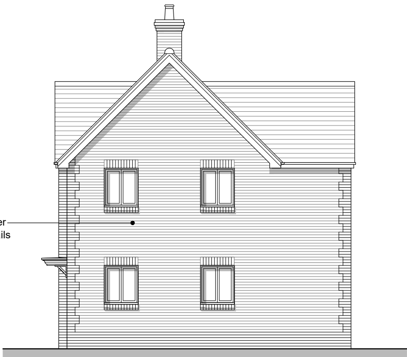
Side Elevation A
