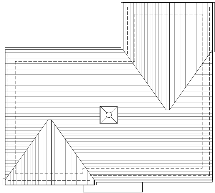
Roof Plan
